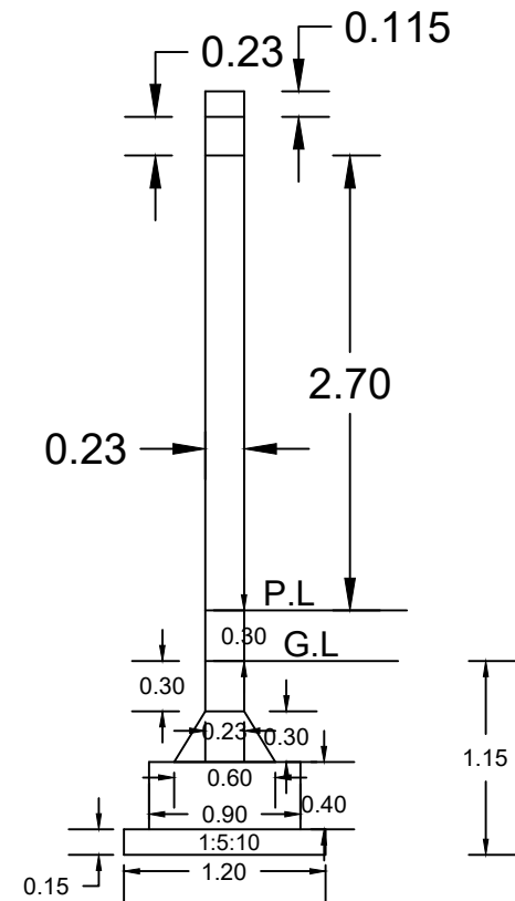
FOUNDATION DETAILS
